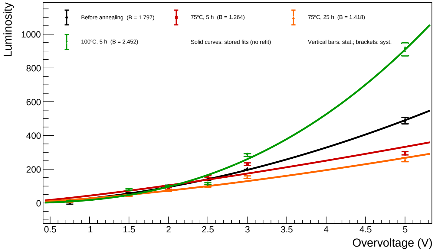
B1_T=20 - Spot 20 ( x = 646.51 , y = 533.37 ): luminosity vs overvoltage for all annealing phases
