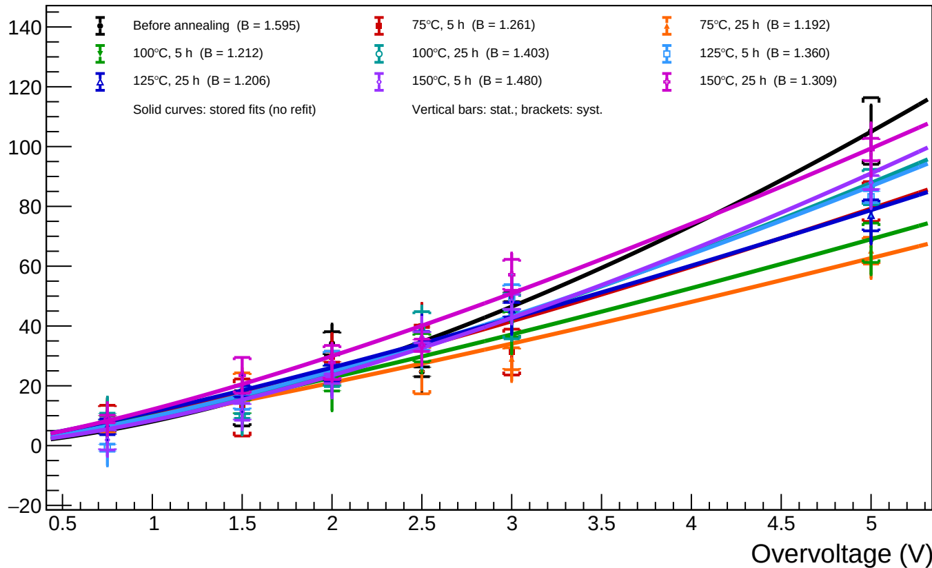
B1_T=20 - Spot 21 (x = 667.70, y = 429.48): luminosity vs overvoltage for all annealing phases
