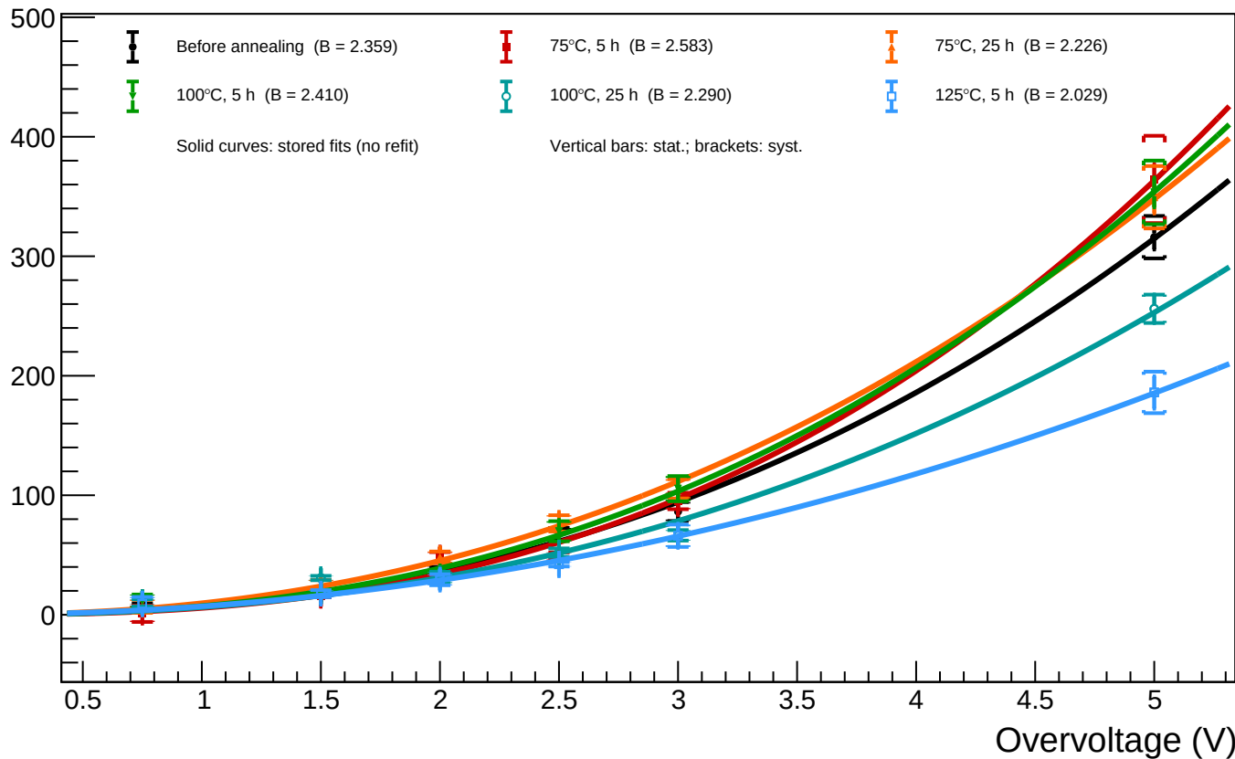
B1_T=20 - Spot 22 (x = 691.50, y = 991.68): luminosity vs overvoltage for all annealing phases
