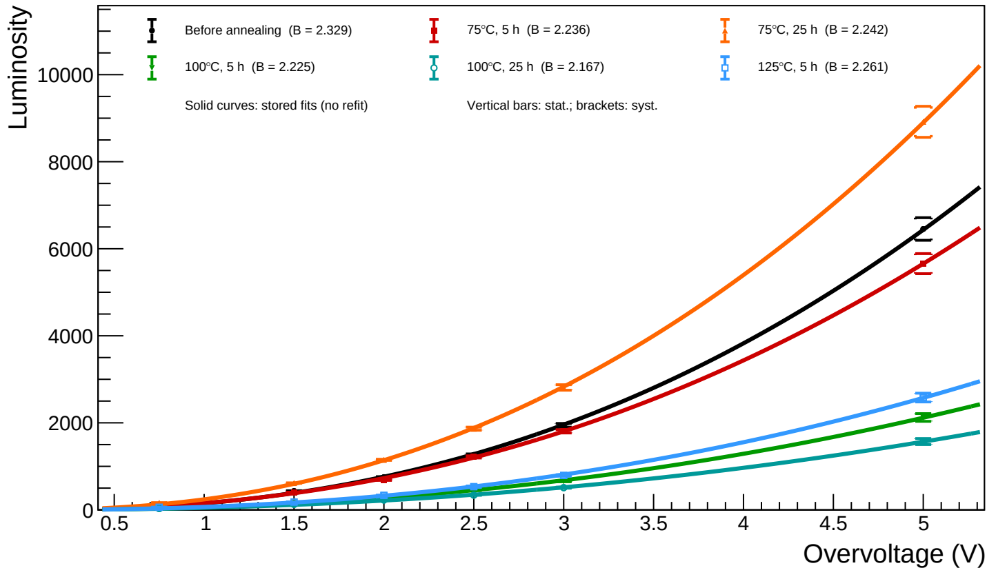
B1_T=20 - Spot 25 ( x = 832.63 , y = 800.65 ): luminosity vs overvoltage for all annealing phases
