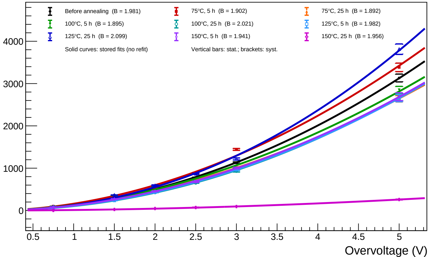
B1_T=20 - Spot 26 ( x = 846.65 , y = 170.33 ): luminosity vs overvoltage for all annealing phases
