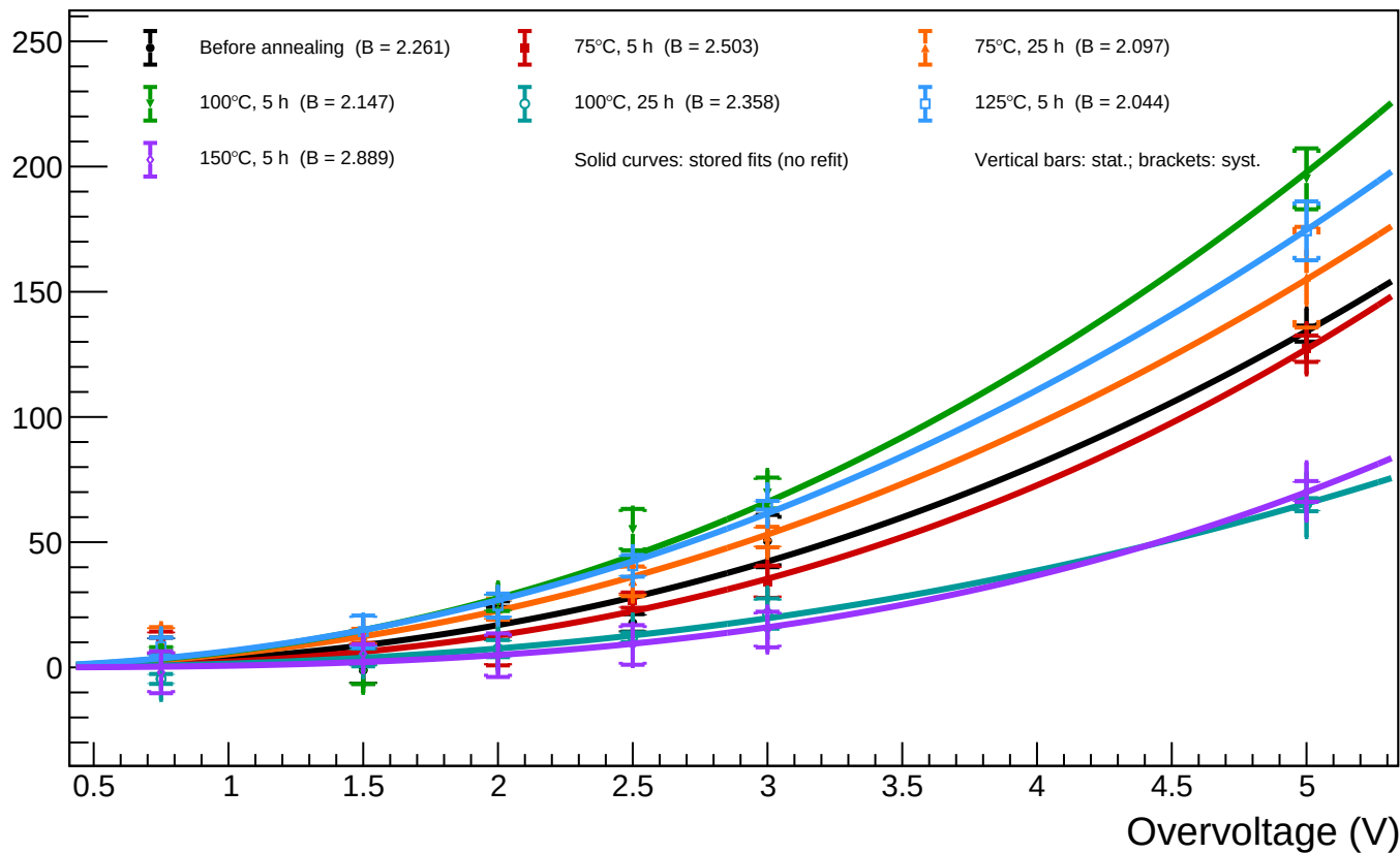
B1_T=20 - Spot 27 ( x = 852.84 , y = 945.13 ): luminosity vs overvoltage for all annealing phases
