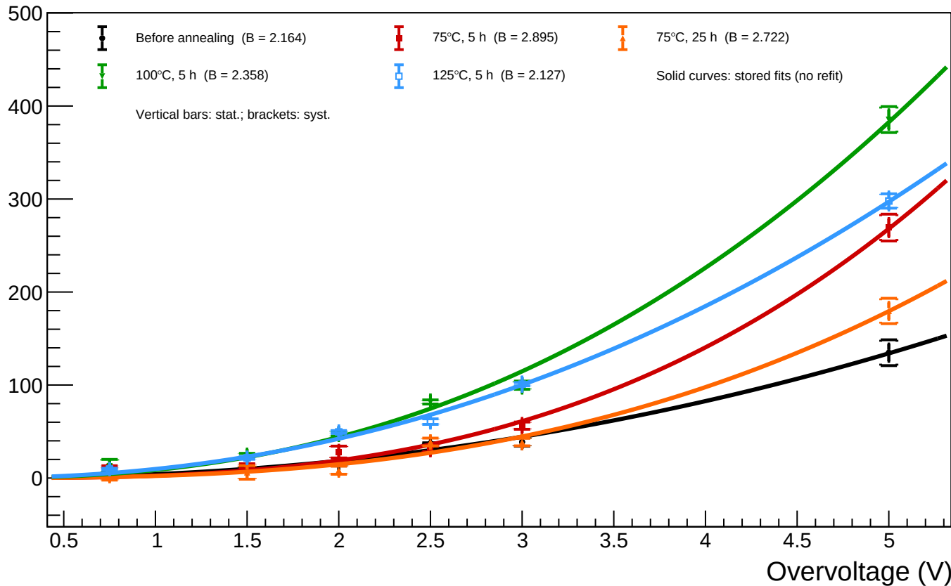
B1_T=20 - Spot 28 ( x = 885.85 , y = 868.93 ): luminosity vs overvoltage for all annealing phases
