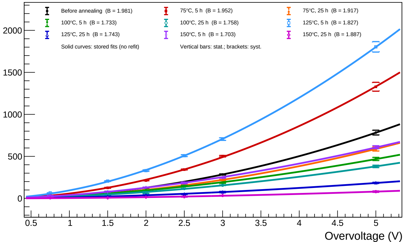
B1_T=20 - Spot 29 ( x = 927.37 , y = 741.36 ): luminosity vs overvoltage for all annealing phases
