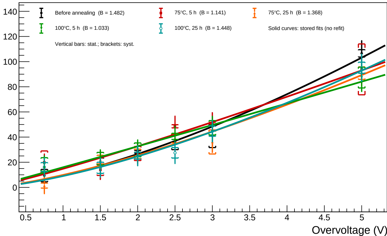
B1_T=20 - Spot 3 (x = 159.62, y = 436.98): luminosity vs overvoltage for all annealing phases
