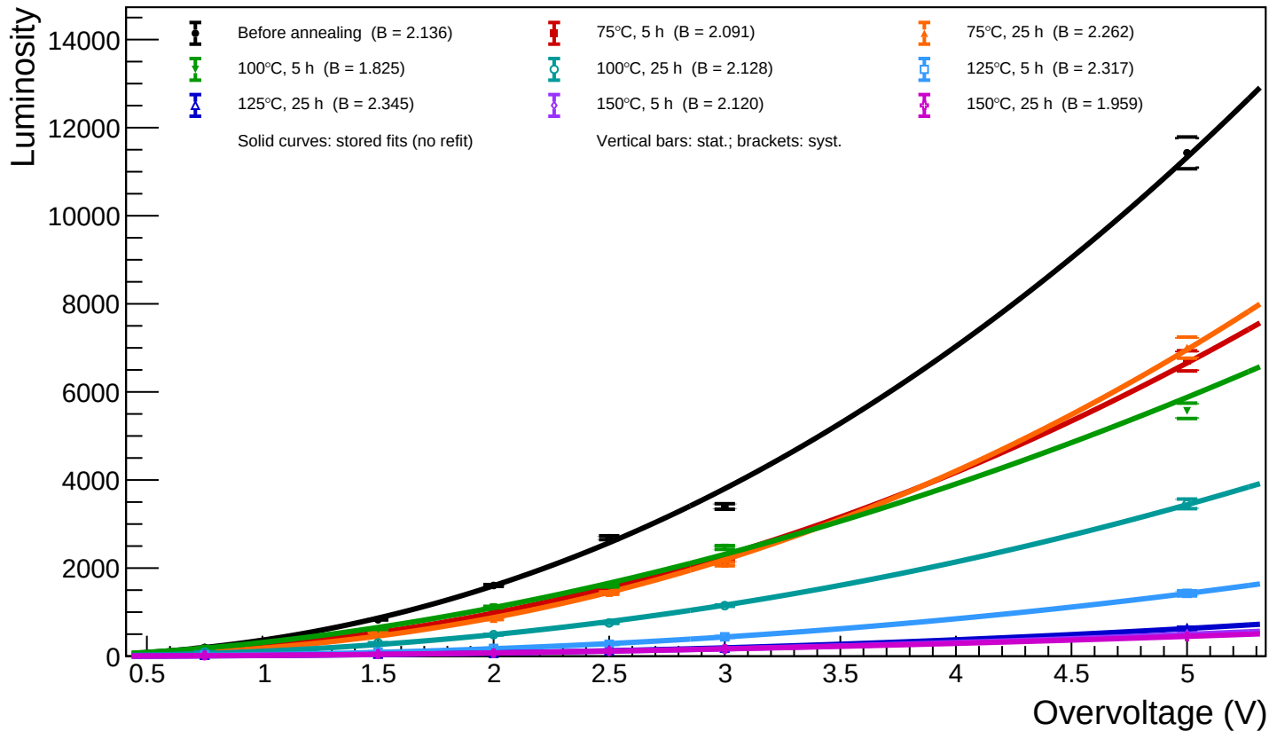
B1_T=20 - Spot 30 ( x = 936.47 , y = 978.99 ): luminosity vs overvoltage for all annealing phases
