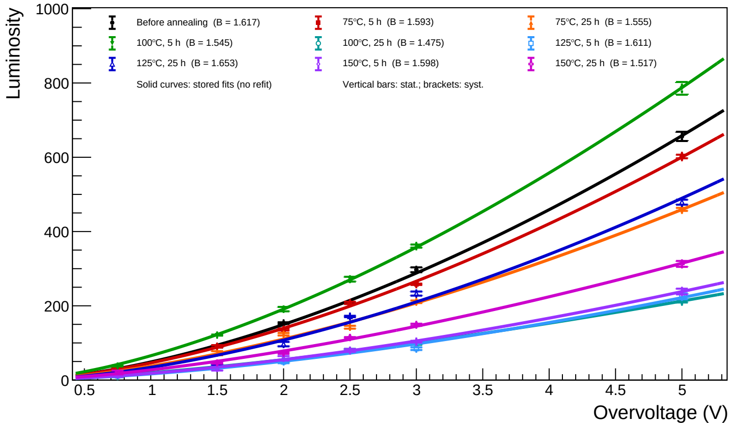
B1_T=20 - Spot 31 ( x = 971.82 , y = 139.53 ): luminosity vs overvoltage for all annealing phases
