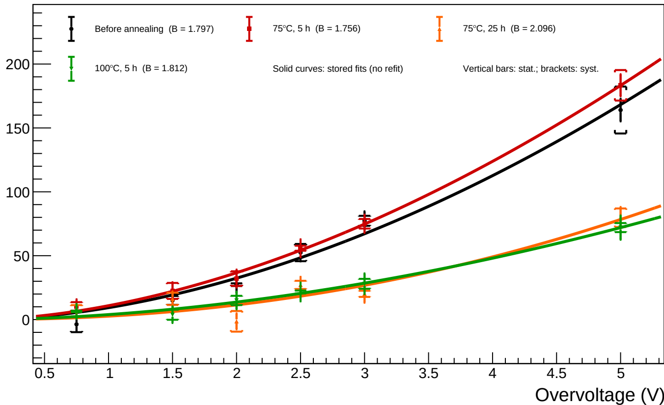
B1_T=20 - Spot 32 ( x = 978.65 , y = 702.64 ): luminosity vs overvoltage for all annealing phases
