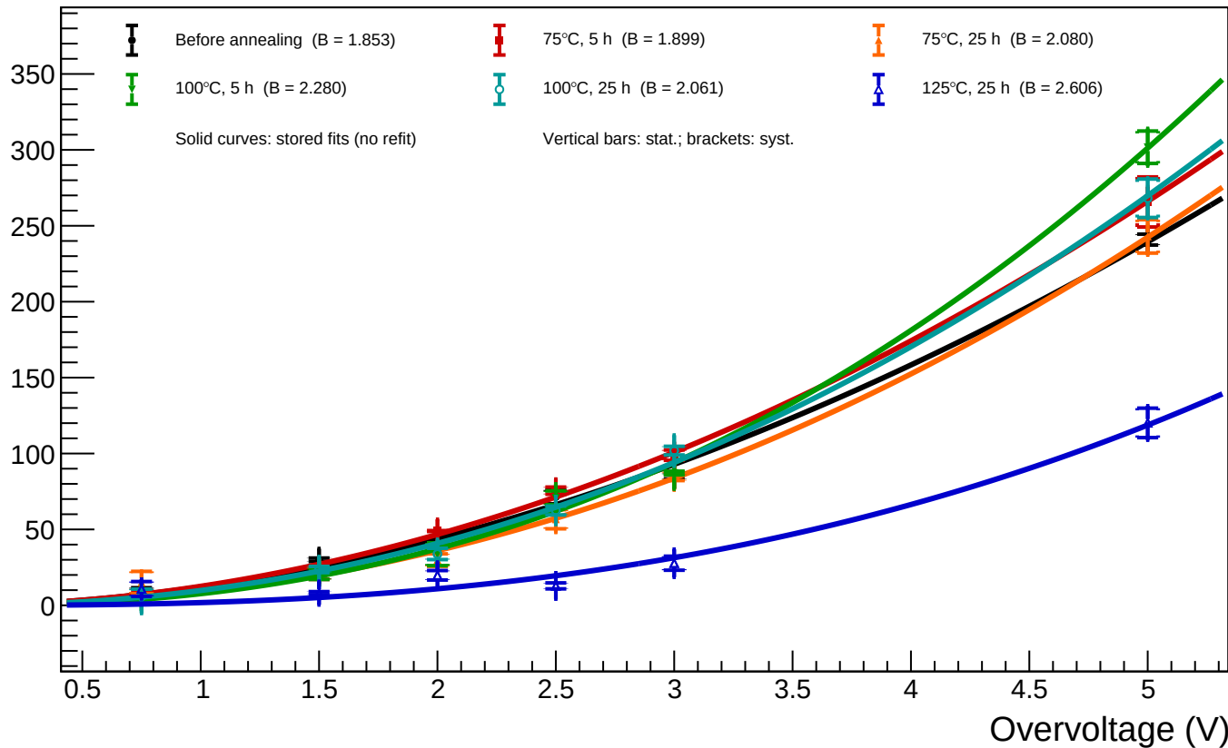
B1_T=20 - Spot 33 (x = 1060.74, y = 683.07): luminosity vs overvoltage for all annealing phases
