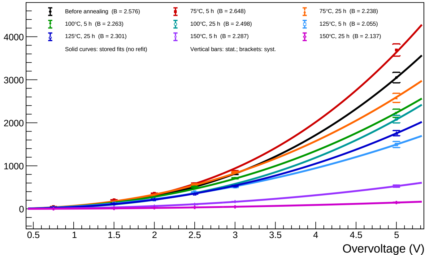
B1_T=20 - Spot 34 (x = 1070.21, y = 854.15): luminosity vs overvoltage for all annealing phases
