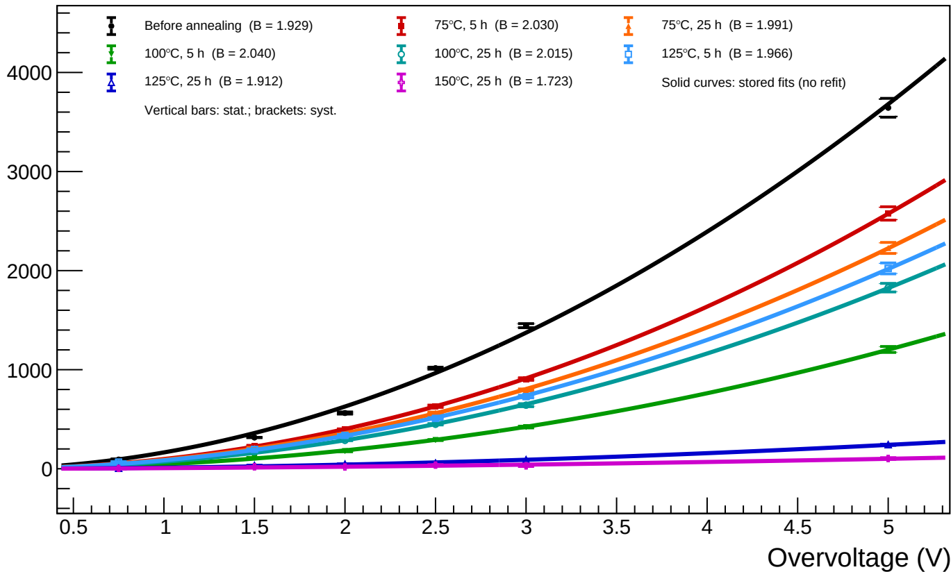
B1_T=20 - Spot 36 (x = 1112.04, y = 793.93): luminosity vs overvoltage for all annealing phases
