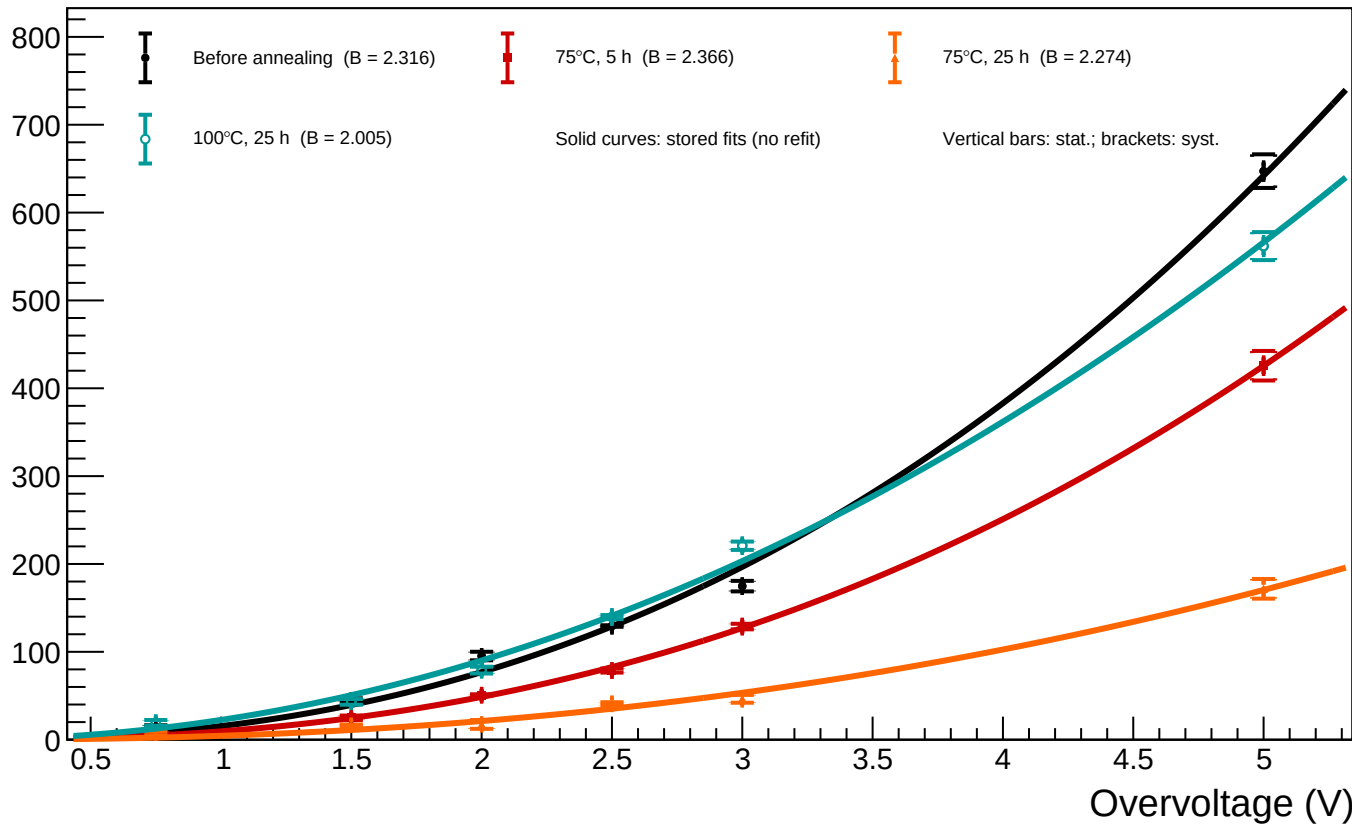
B1_T=20 - Spot 37 (x = 1121.09, y = 918.20): luminosity vs overvoltage for all annealing phases
