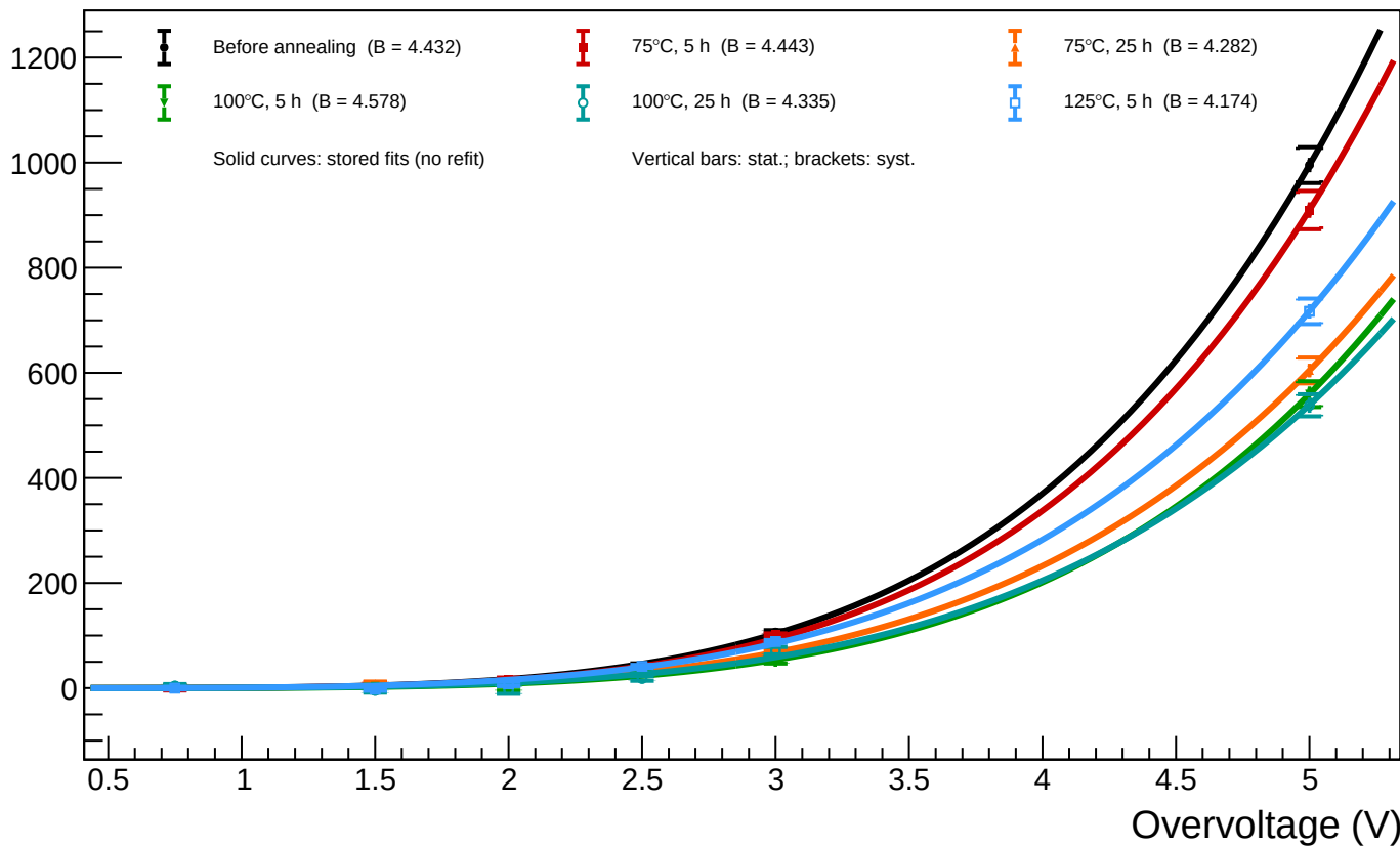
B1_T=20 - Spot 38 (x = 1189.24, y = 757.61): luminosity vs overvoltage for all annealing phases
