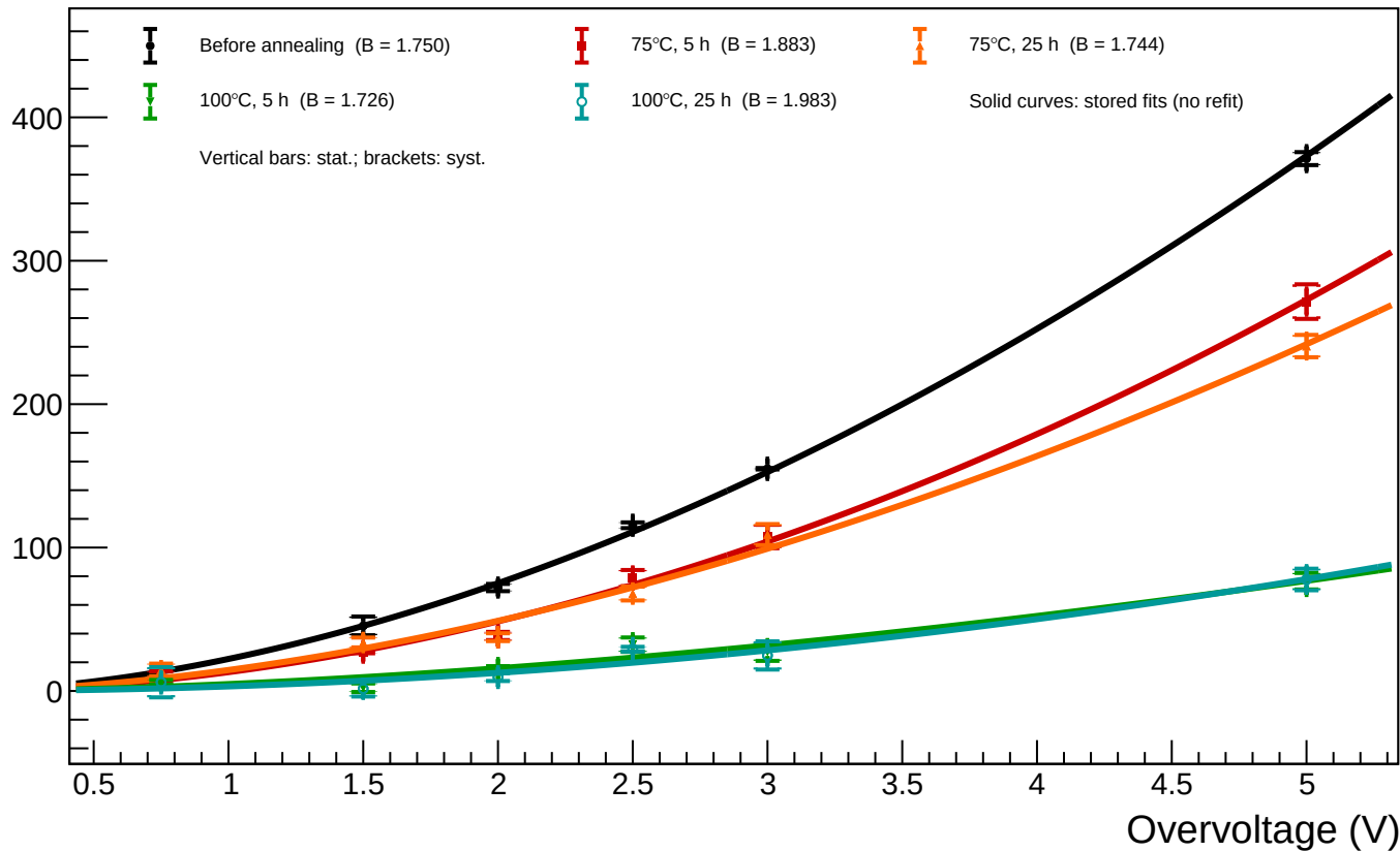
B1_T=20 - Spot 39 (x = 1218.02, y = 693.08): luminosity vs overvoltage for all annealing phases
