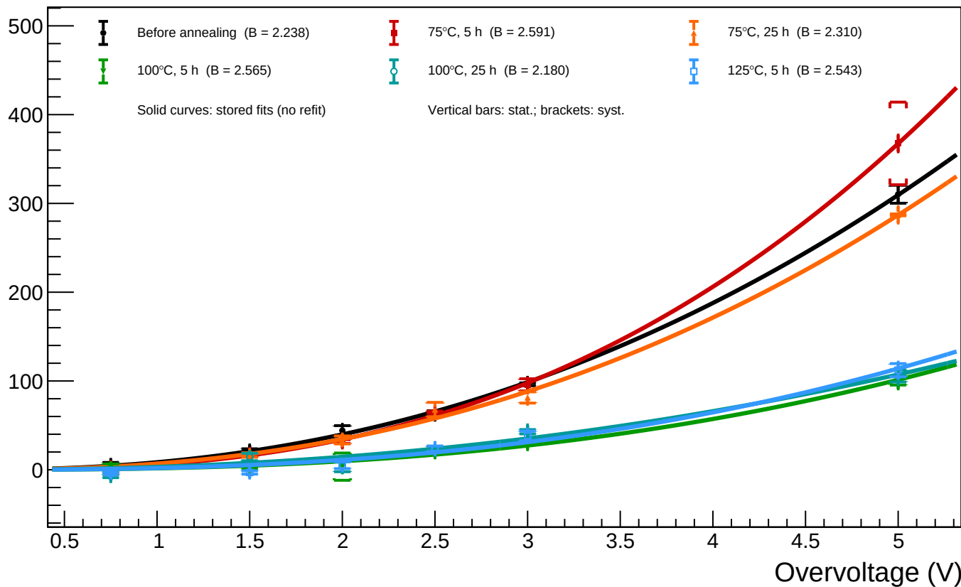
B1_T=20 - Spot 4 (x = 206.32, y = 892.43): luminosity vs overvoltage for all annealing phases
