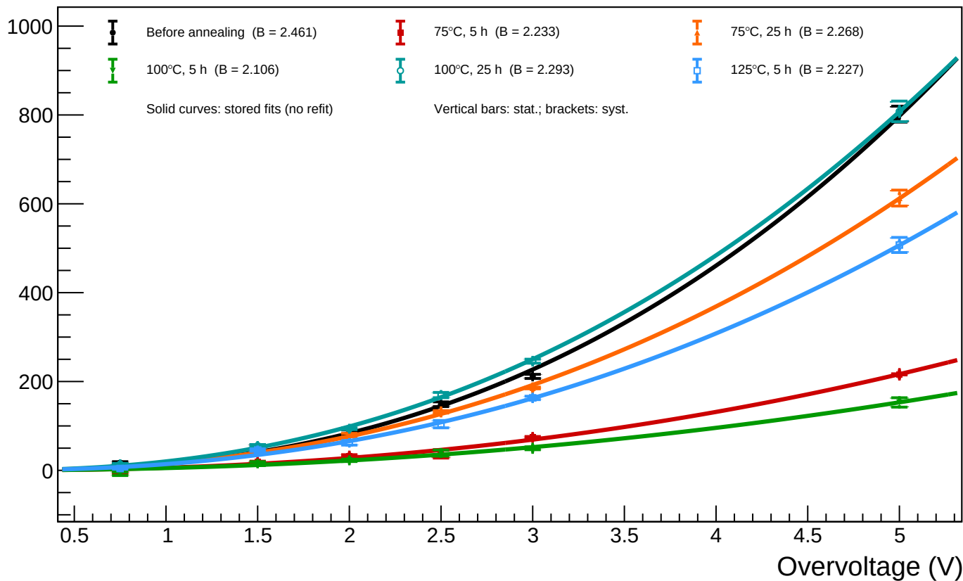
B1_T=20 - Spot 40 ( x = 1226.31 , y = 80.11 ): luminosity vs overvoltage for all annealing phases
