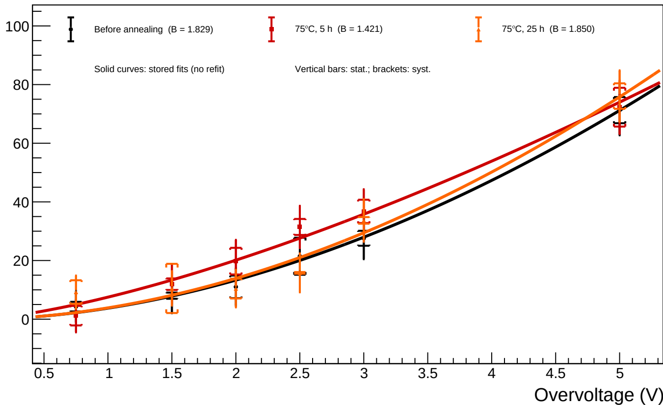
B1_T=20 - Spot 41 (x = 1269.96, y = 982.07): luminosity vs overvoltage for all annealing phases
