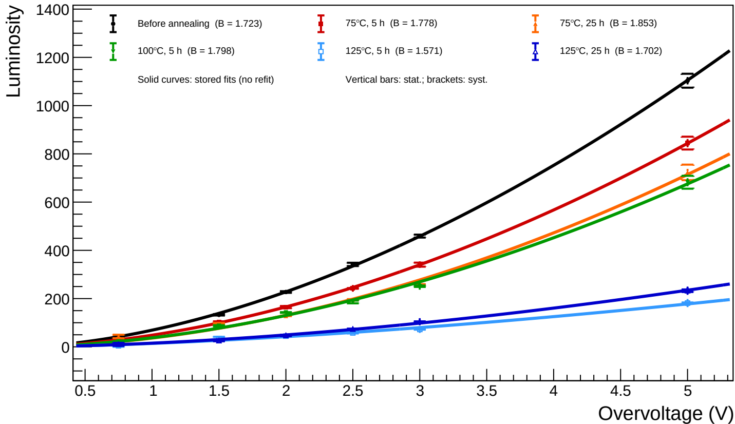
B1_T=20 - Spot 42 (x = 1278.47, y = 556.41): luminosity vs overvoltage for all annealing phases
