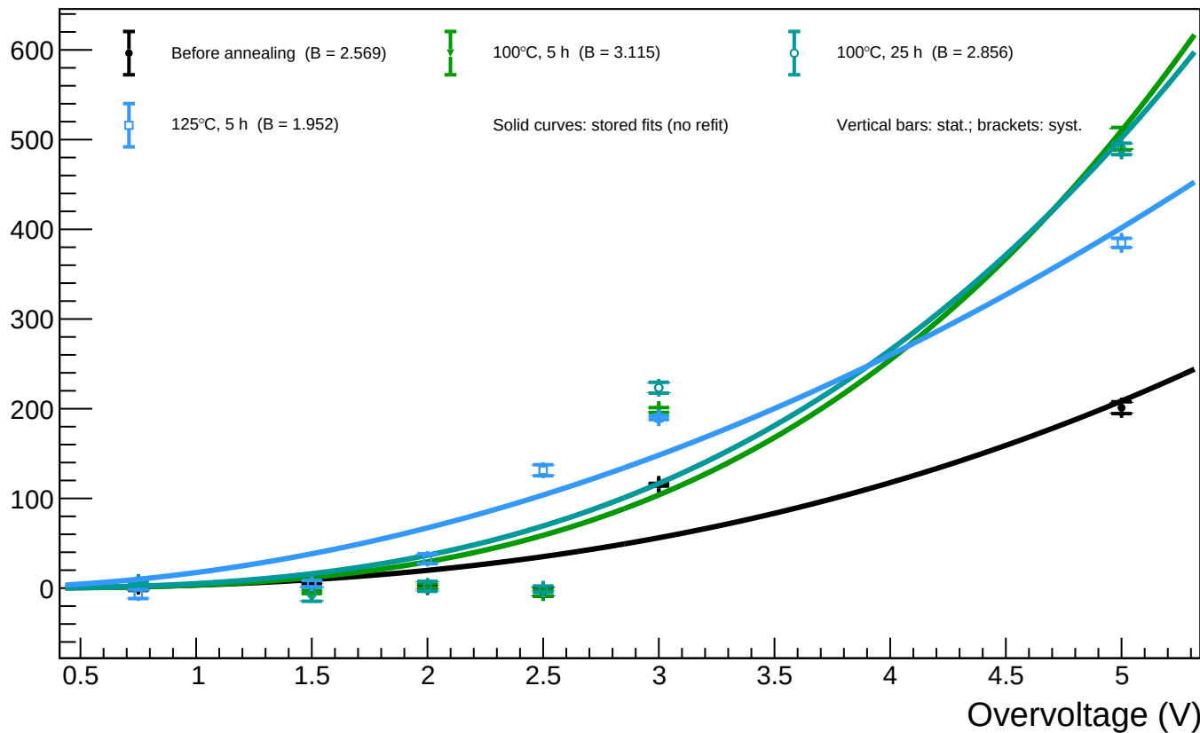
B1_T=20 - Spot 43 (x = 1344.99, y = 131.83): luminosity vs overvoltage for all annealing phases
