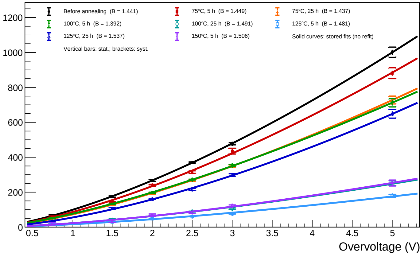
B1_T=20 - Spot 45 (x = 1401.61, y = 766.05): luminosity vs overvoltage for all annealing phases
