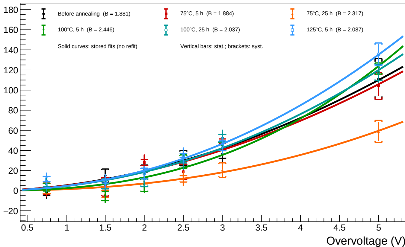
B1_T=20 - Spot 46 (x = 1466.69, y = 874.64): luminosity vs overvoltage for all annealing phases
