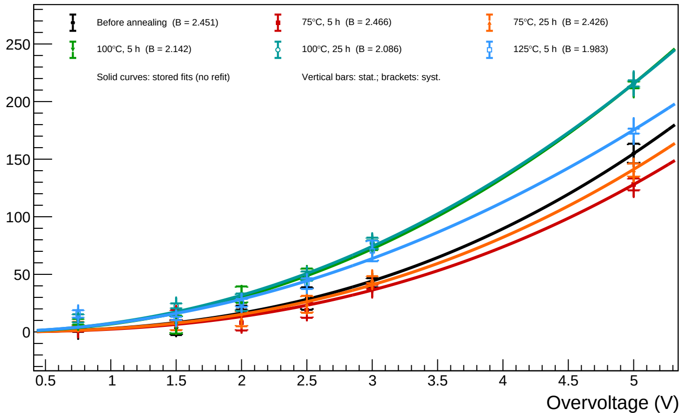
B1_T=20 - Spot 48 (x = 1503.43, y = 978.17): luminosity vs overvoltage for all annealing phases
