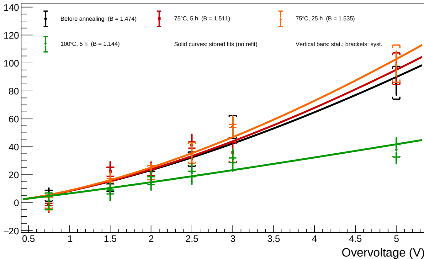
B1_T=20 - Spot 49 (x = 1506.19, y = 229.87): luminosity vs overvoltage for all annealing phases
