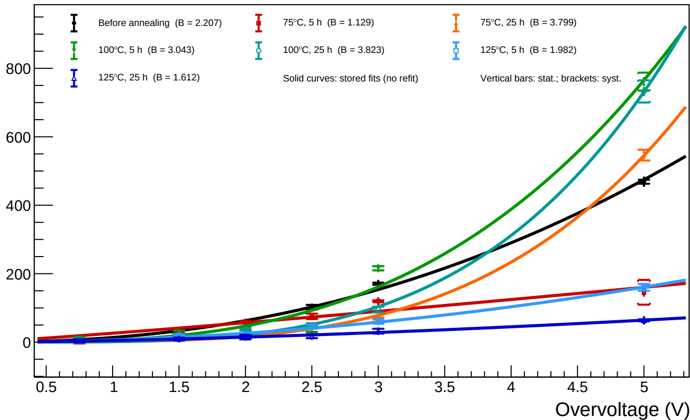
B1_T=20 - Spot 5 (x = 217.60, y = 313.79): luminosity vs overvoltage for all annealing phases
