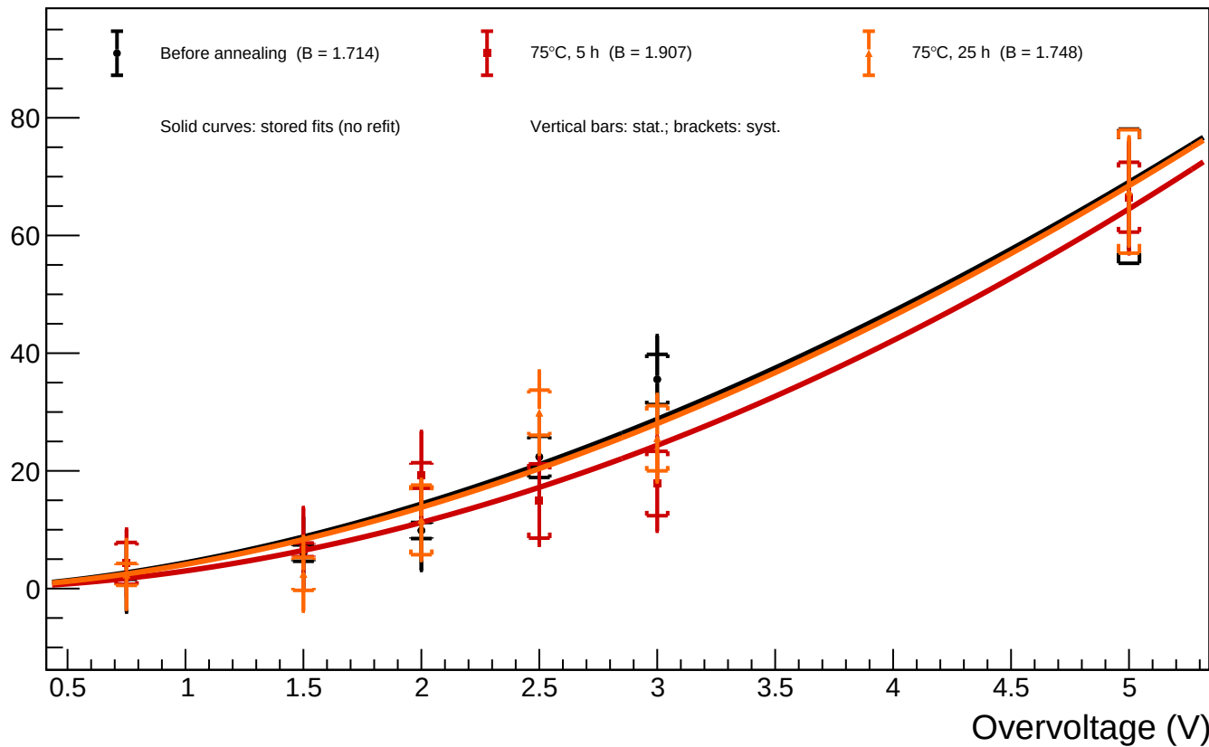
B1_T=20 - Spot 50 (x = 1558.35, y = 609.07): luminosity vs overvoltage for all annealing phases
