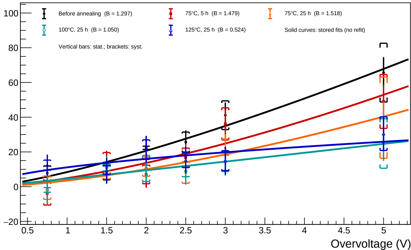
B1_T=20 - Spot 51 (x = 1587.59, y = 278.57): luminosity vs overvoltage for all annealing phases
