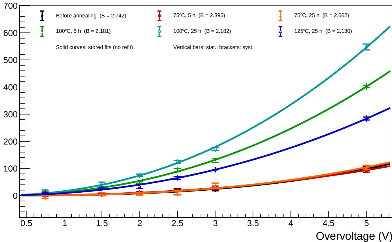
B1_T=20 - Spot 52 ( x = 1628.53 , y = 86.35 ): luminosity vs overvoltage for all annealing phases
