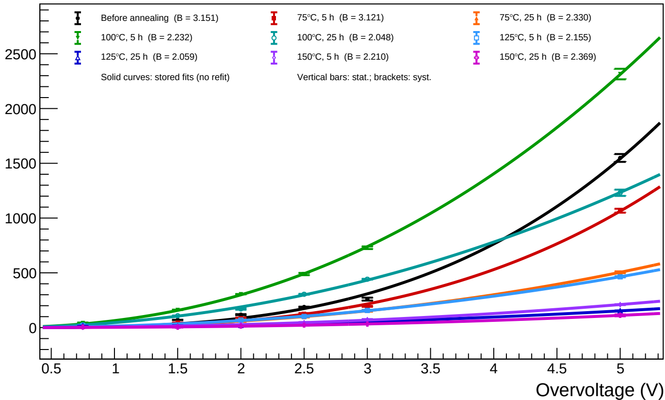
B1_T=20 - Spot 53 (x = 1685.63, y = 913.87): luminosity vs overvoltage for all annealing phases
