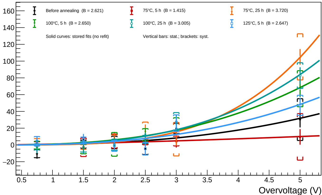
B1_T=20 - Spot 54 (x = 1709.11, y = 446.55): luminosity vs overvoltage for all annealing phases
