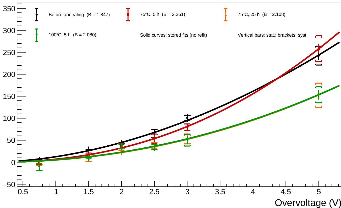
B1_T=20 - Spot 55 (x = 1711.52, y = 373.64): luminosity vs overvoltage for all annealing phases
