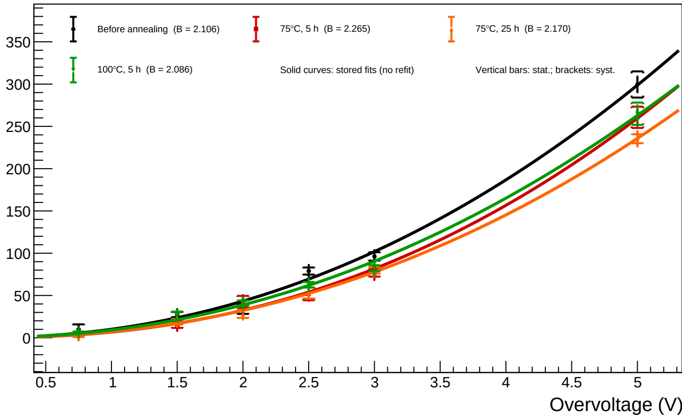
B1_T=20 - Spot 56 (x = 1753.66, y = 201.94): luminosity vs overvoltage for all annealing phases
