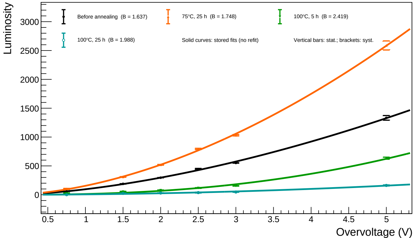
B1_T=20 - Spot 59 (x = 1820.96, y = 987.39): luminosity vs overvoltage for all annealing phases
