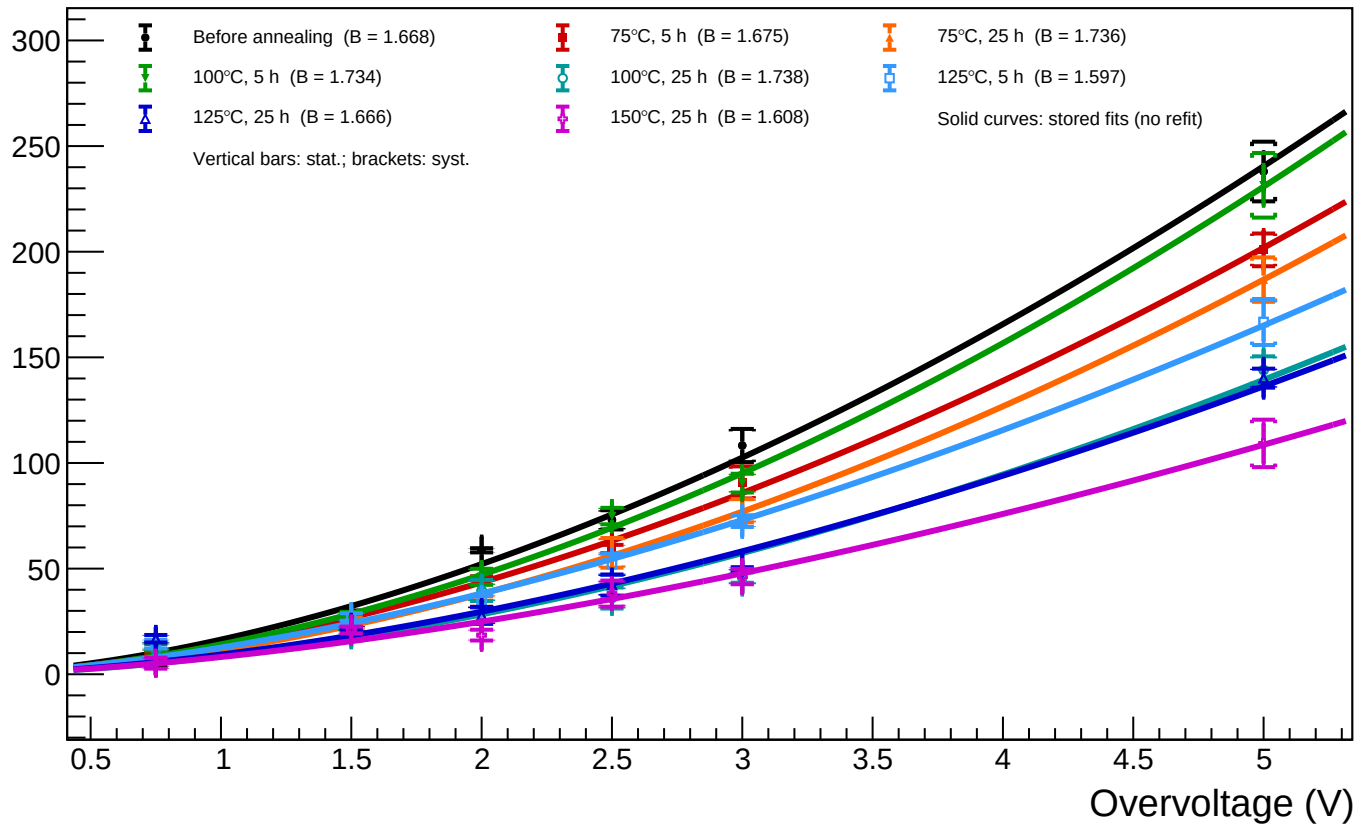
B1_T=20 - Spot 6 (x = 234.25, y = 476.95): luminosity vs overvoltage for all annealing phases
