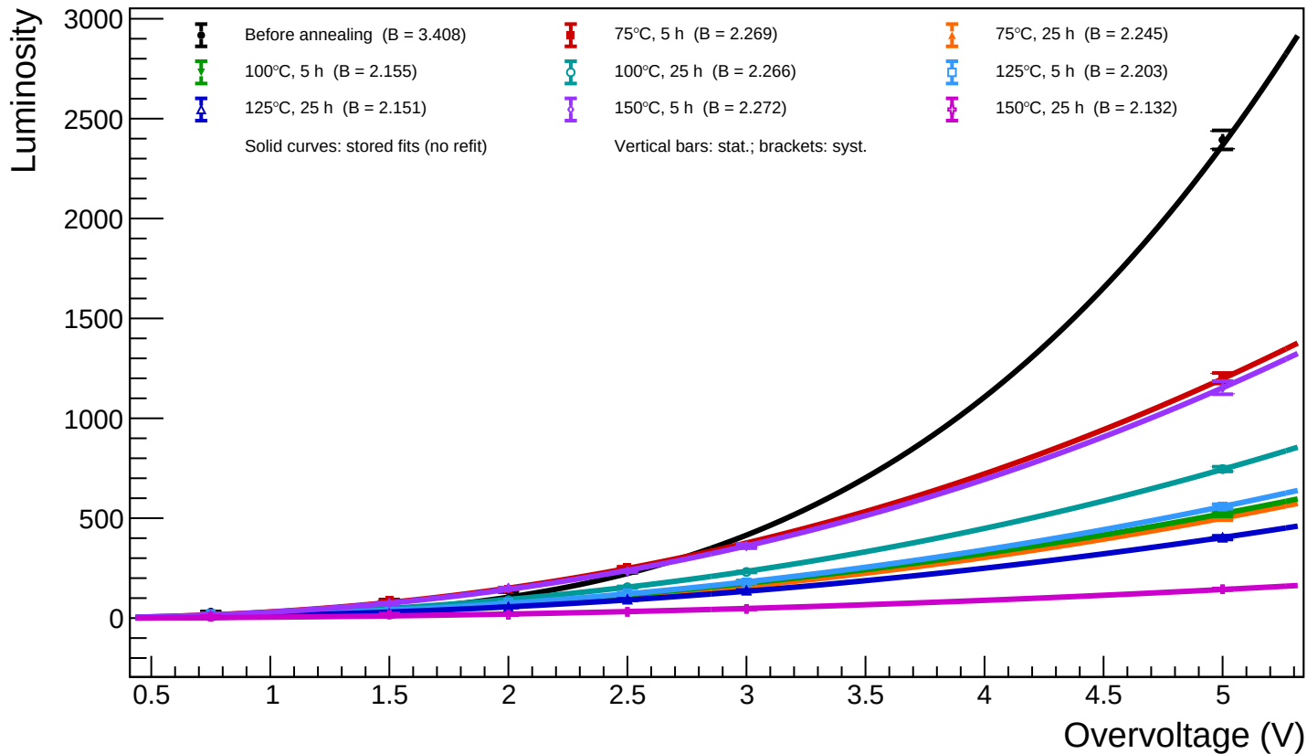
B1_T=20 - Spot 60 (x = 1832.27, y = 271.51): luminosity vs overvoltage for all annealing phases
