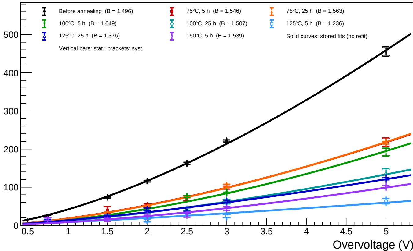
B1_T=20 - Spot 61 (x = 1841.56, y = 811.07): luminosity vs overvoltage for all annealing phases
