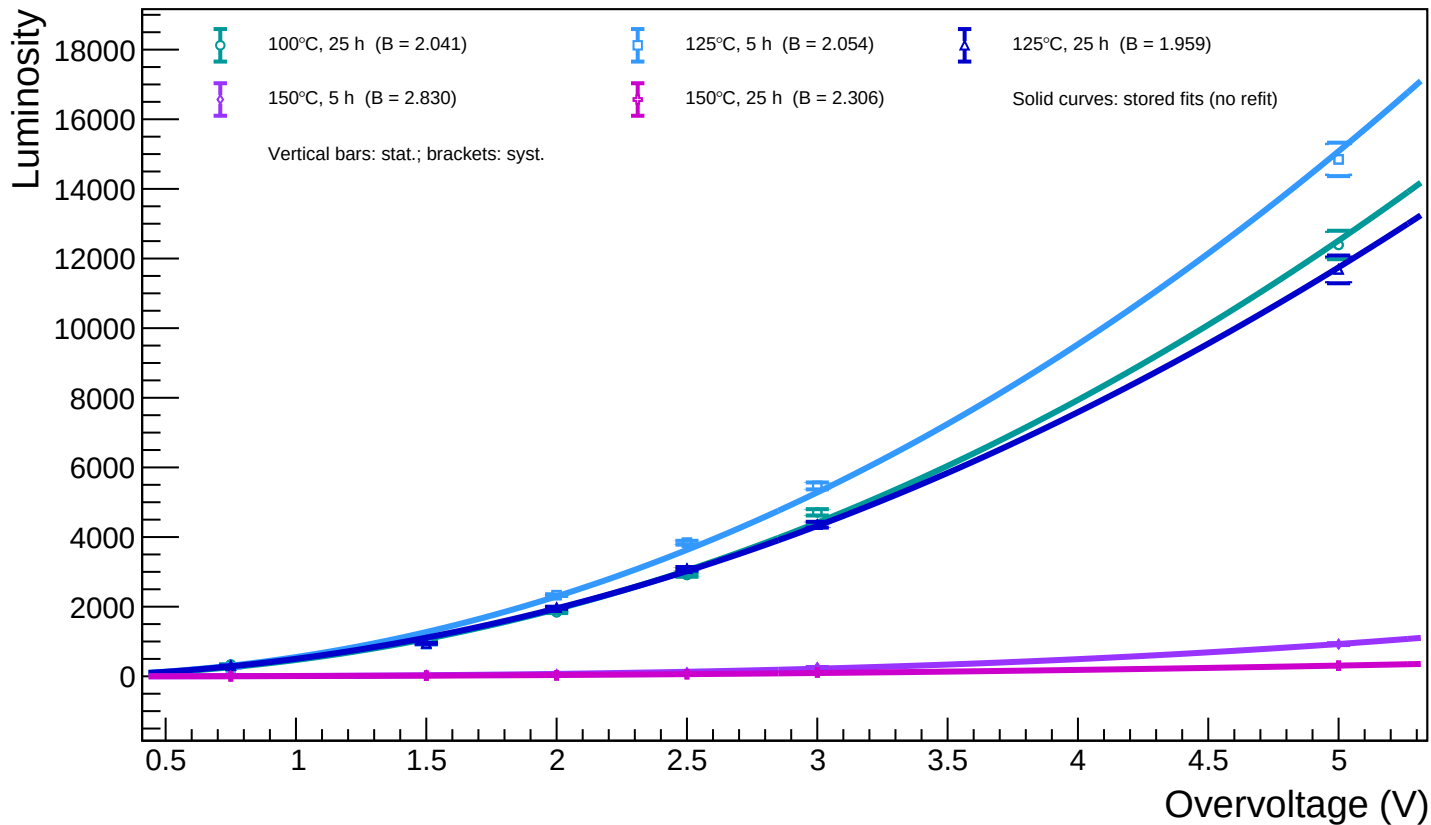
B1_T=20 - Spot 63 ( x = 452.08 , y = 609.35 ): luminosity vs overvoltage for all annealing phases
