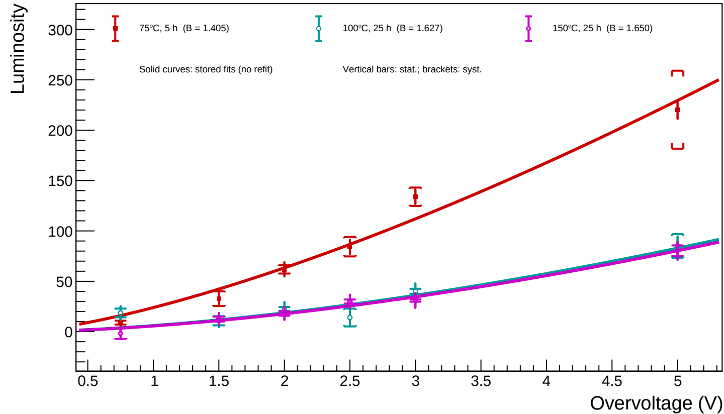
B1_T=20 - Spot 64 ( x = 464.27 , y = 404.00 ): luminosity vs overvoltage for all annealing phases
