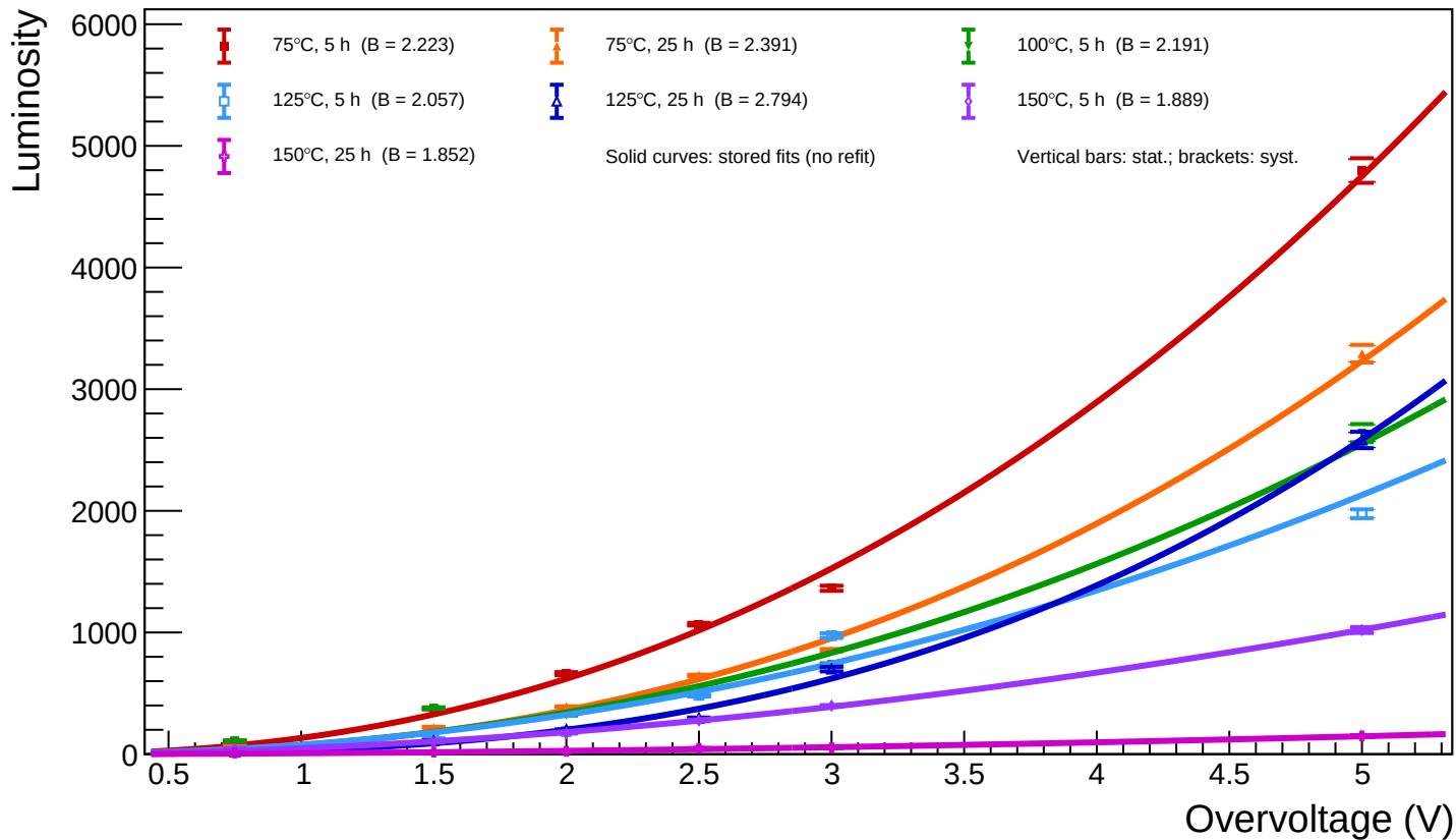
B1_T=20 - Spot 65 (x = 503.75, y = 521.81): luminosity vs overvoltage for all annealing phases
