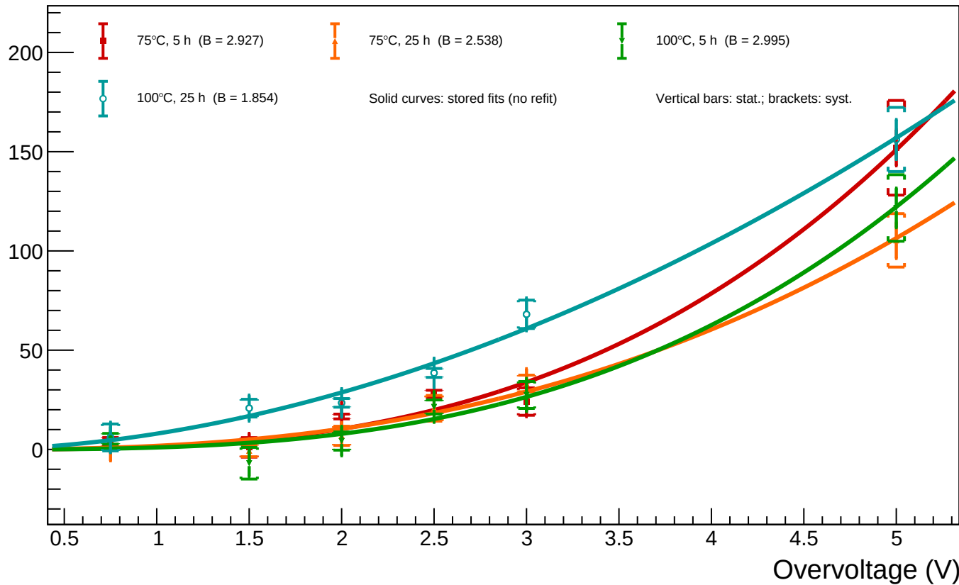
B1_T=20 - Spot 67 ( x = 983.87 , y = 928.54 ): luminosity vs overvoltage for all annealing phases
