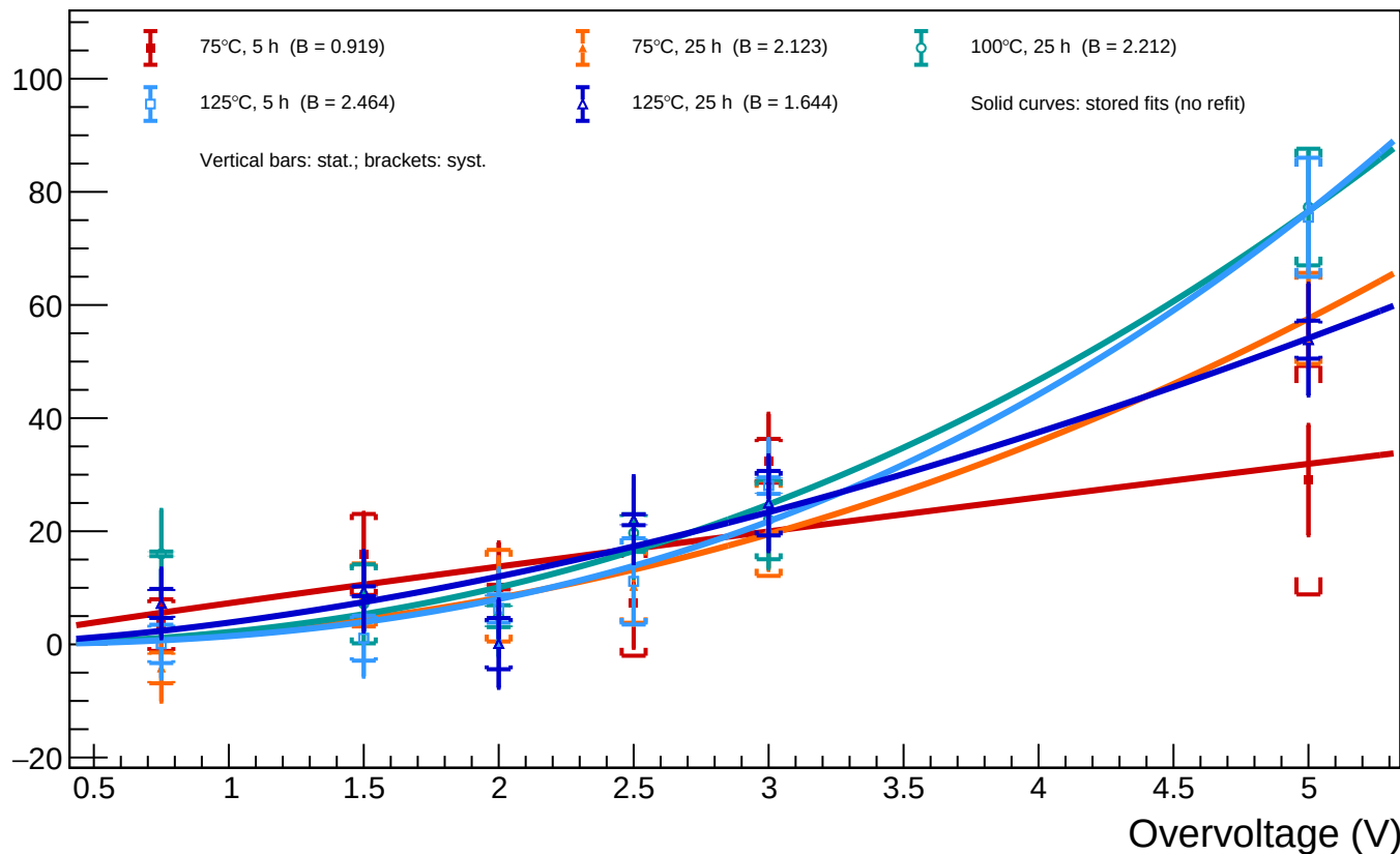
B1_T=20 - Spot 68 (x = 1202.73, y = 204.44): luminosity vs overvoltage for all annealing phases
