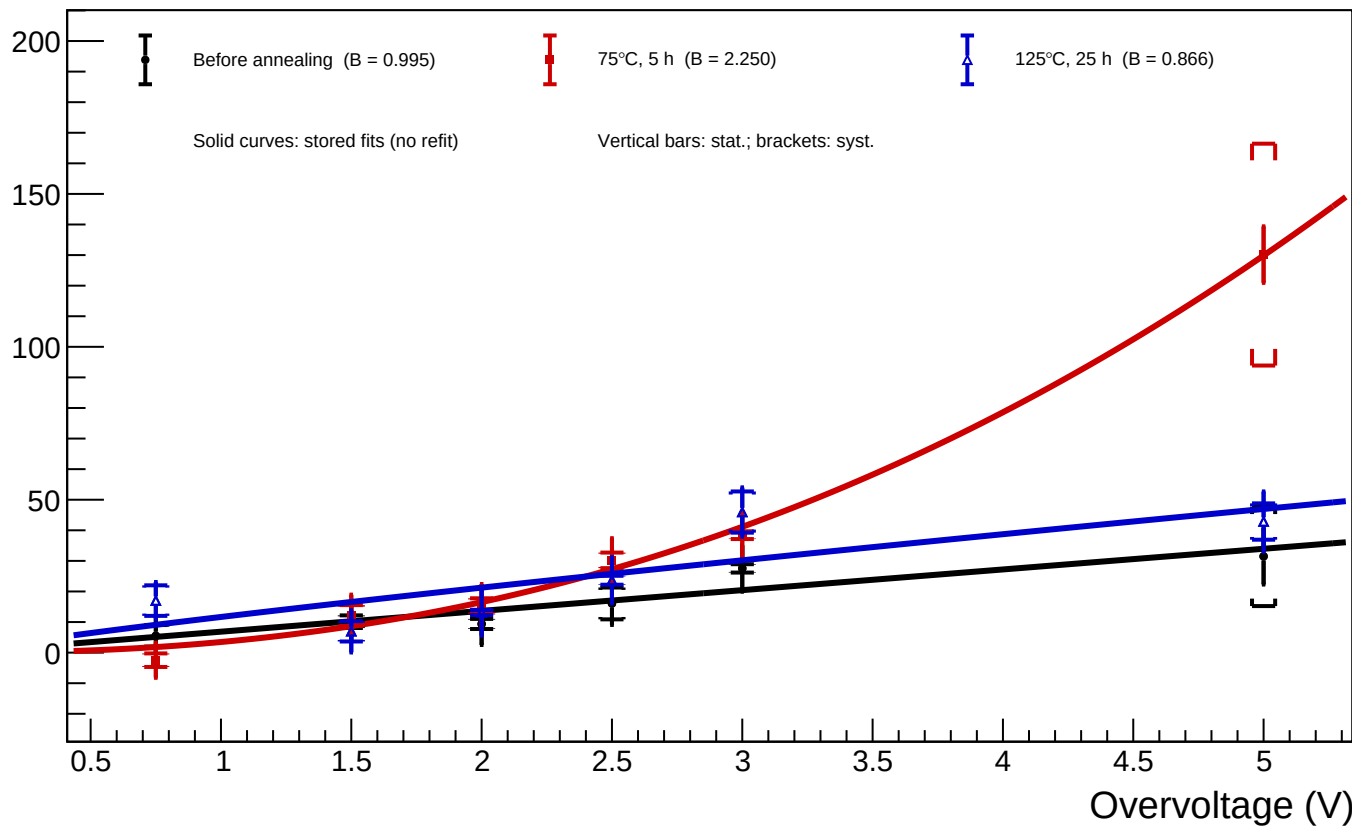
B1_T=20 - Spot 7 (x = 281.02, y = 945.86): luminosity vs overvoltage for all annealing phases
