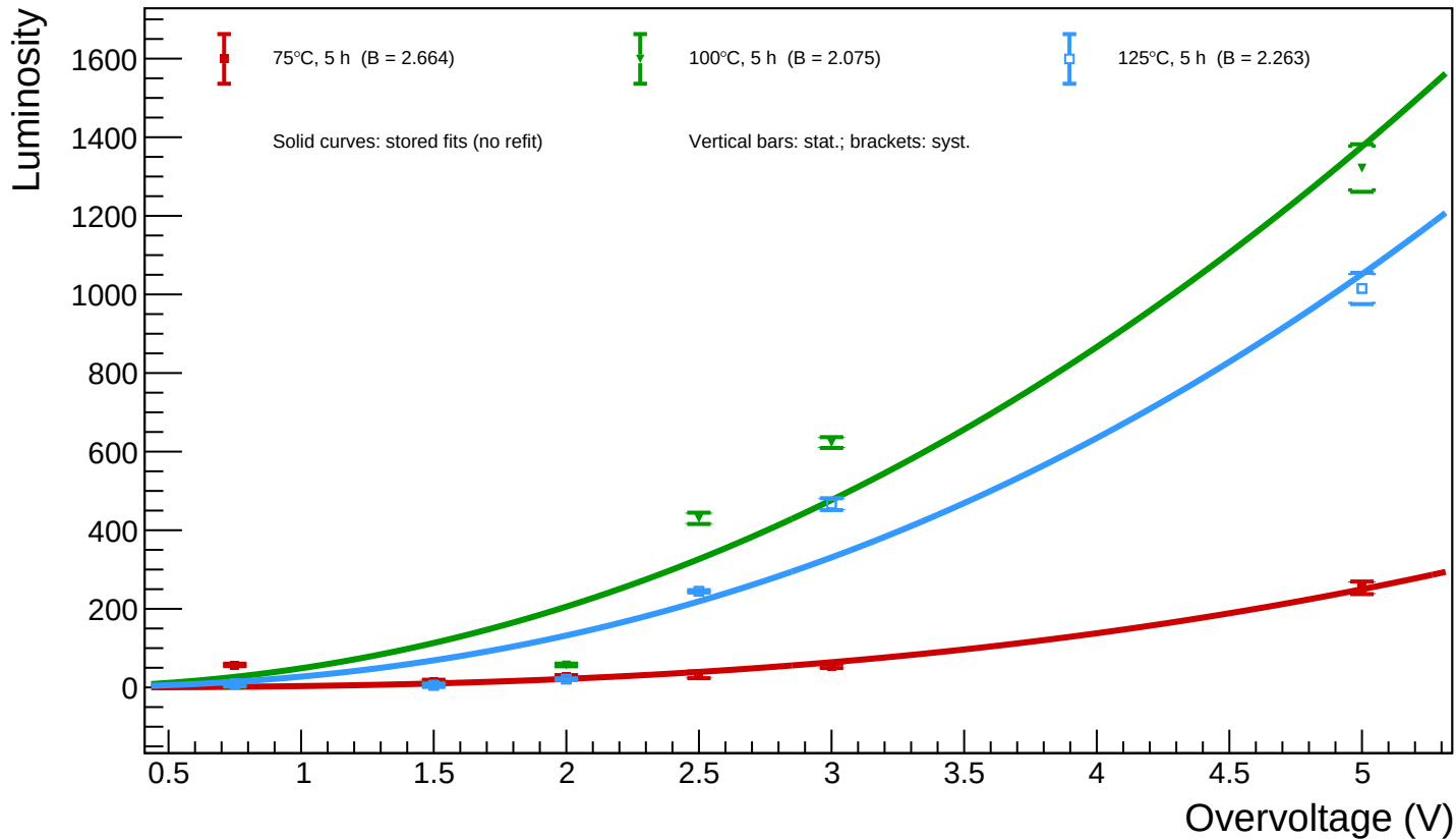
B1_T=20 - Spot 70 ( x = 148.83 , y = 605.35 ): luminosity vs overvoltage for all annealing phases
