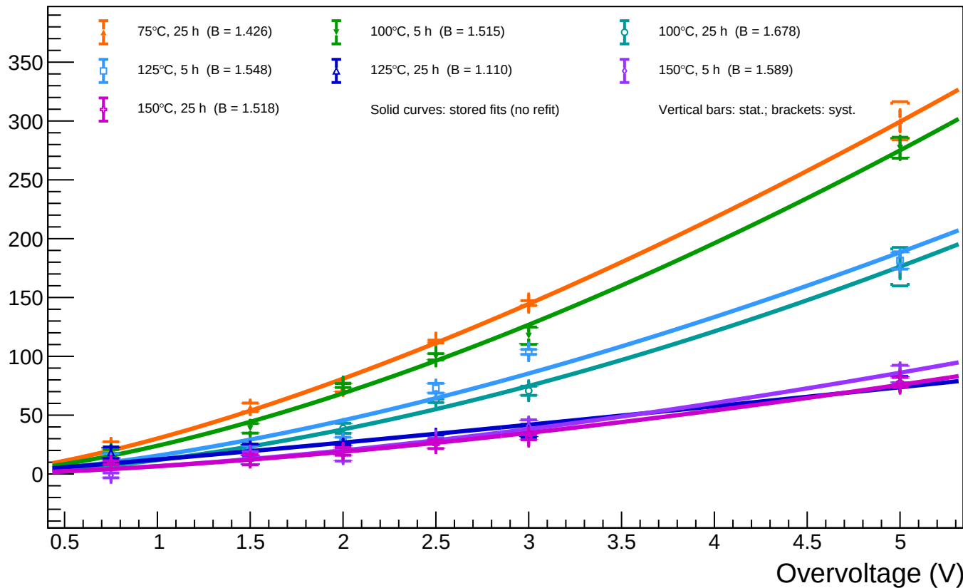
B1_T=20 - Spot 74 ( x = 791.92 , y = 460.46 ): luminosity vs overvoltage for all annealing phases
