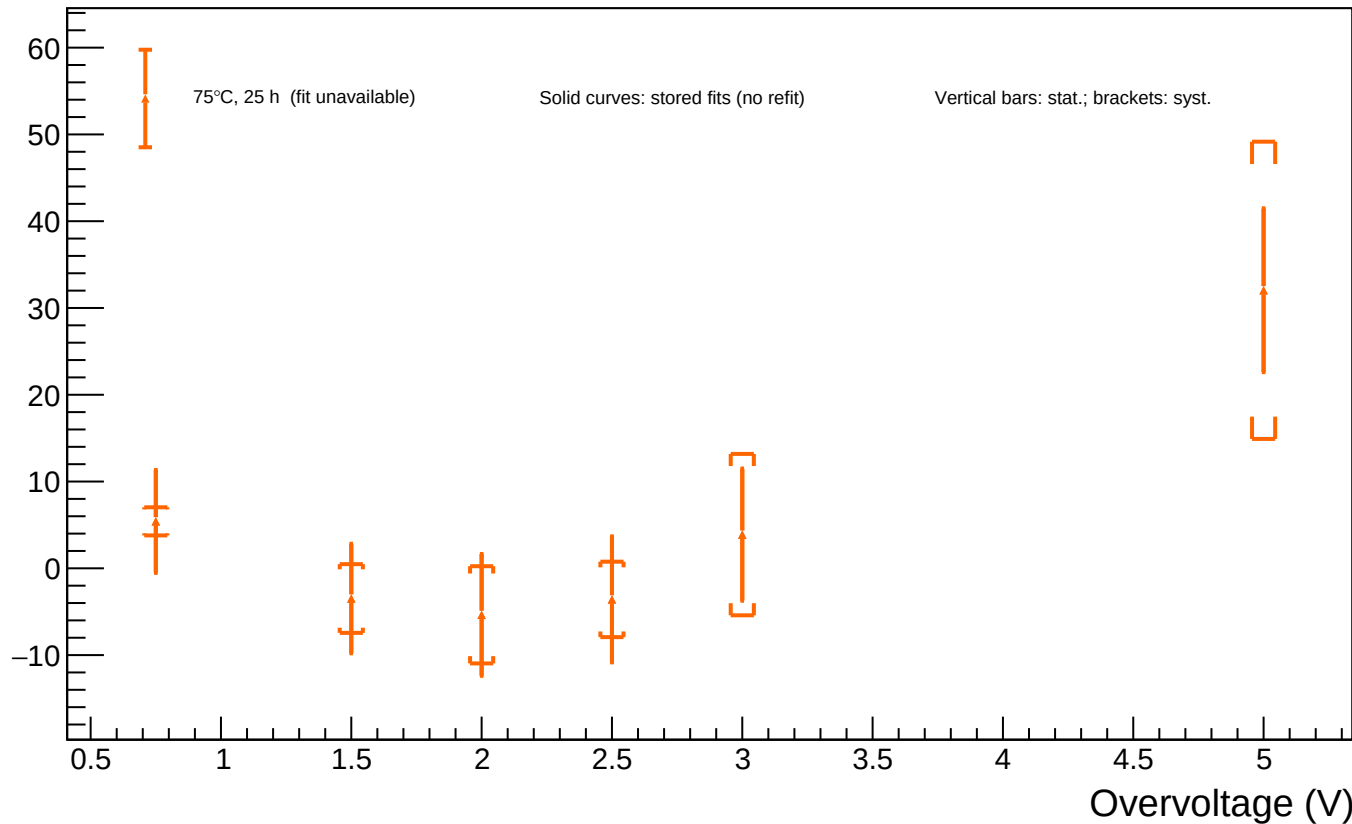
B1_T=20 - Spot 79 (x = 1585.57, y = 548.25): luminosity vs overvoltage for all annealing phases
