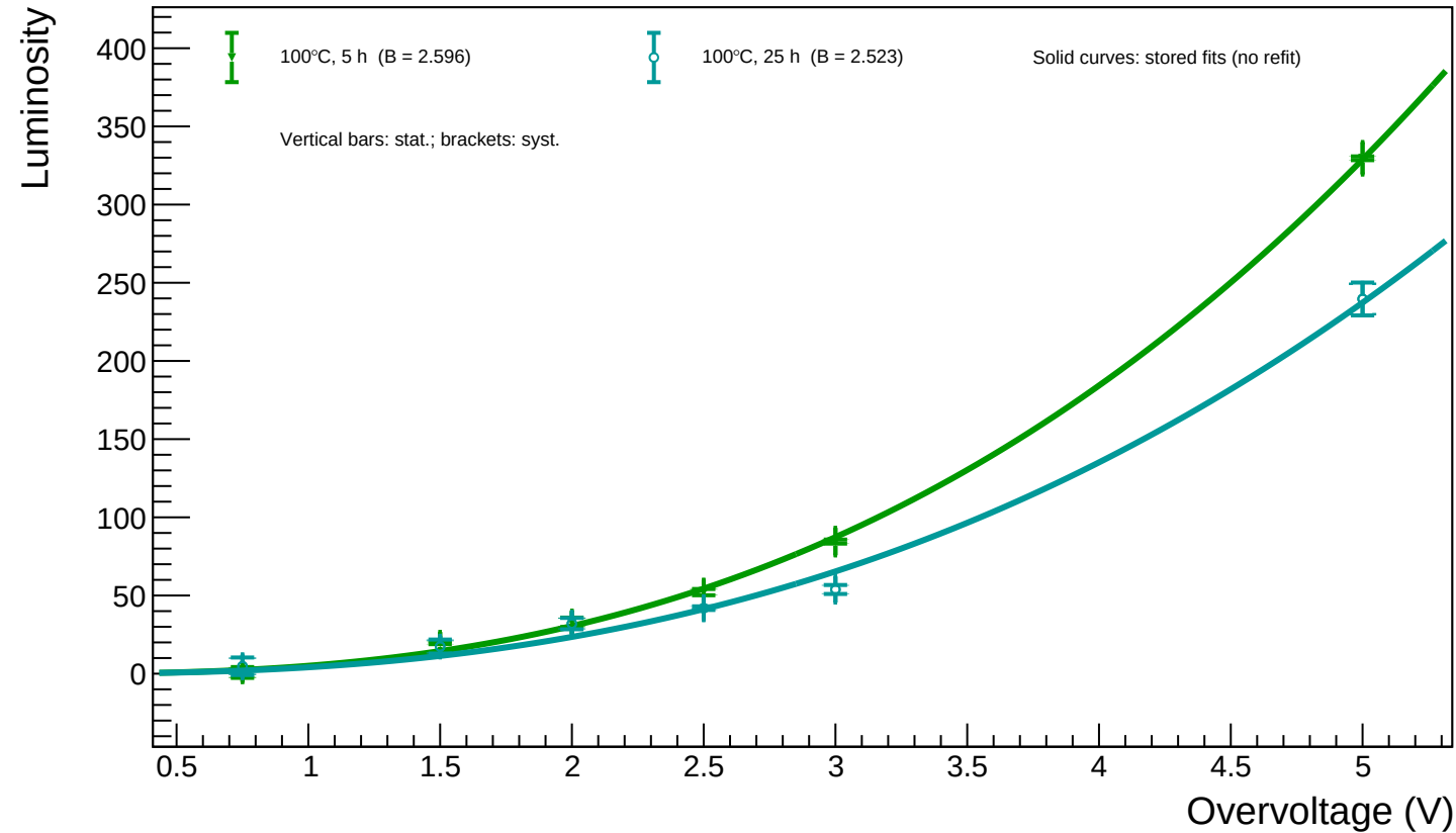
B1_T=20 - Spot 80 ( x = 713.40 , y = 108.75 ): luminosity vs overvoltage for all annealing phases
