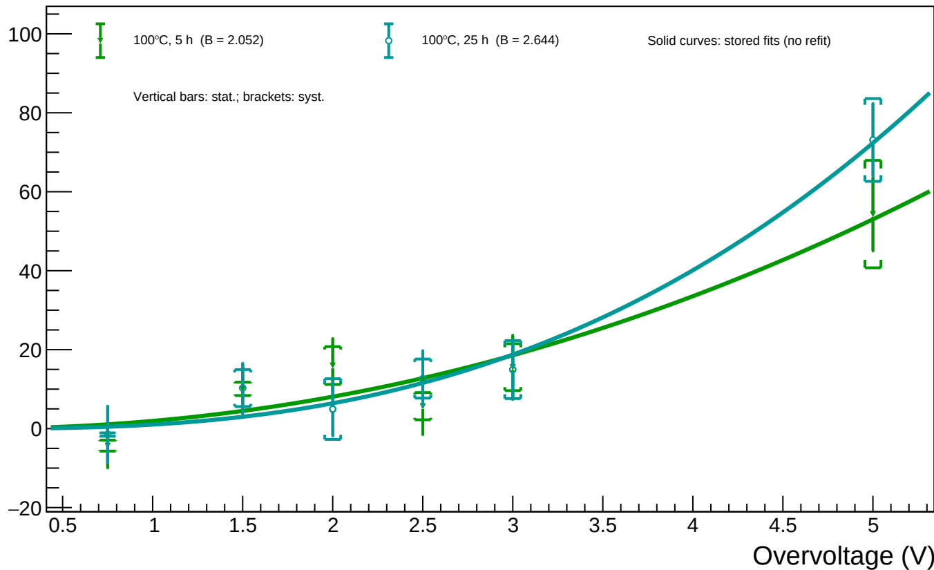
B1_T=20 - Spot 82 (x = 1442.44, y = 321.69): luminosity vs overvoltage for all annealing phases
